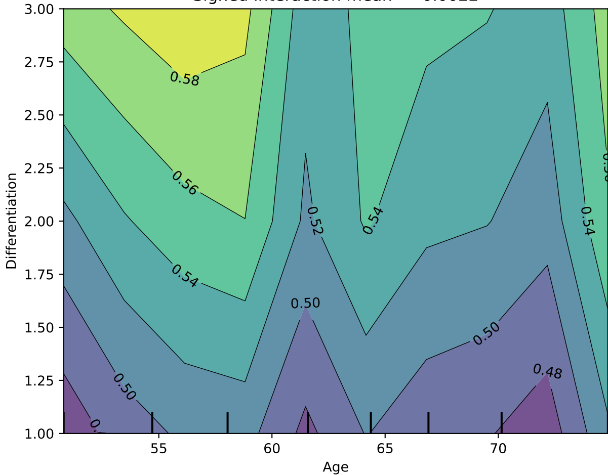
2D PDP: Age \times Differentiation Signed interaction mean = -0.0022
