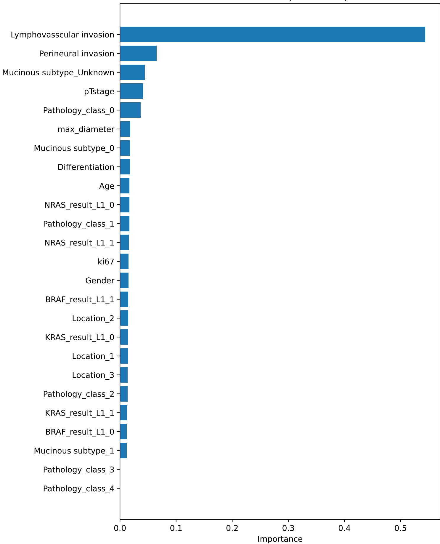
XGBoost Feature Importance Top 30
