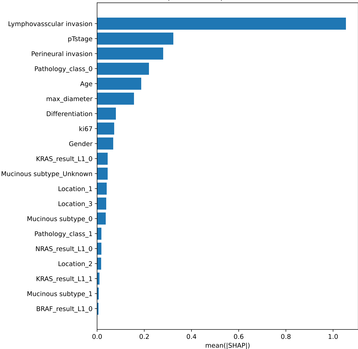
Top 20 SHAP Importance - XGBoost
