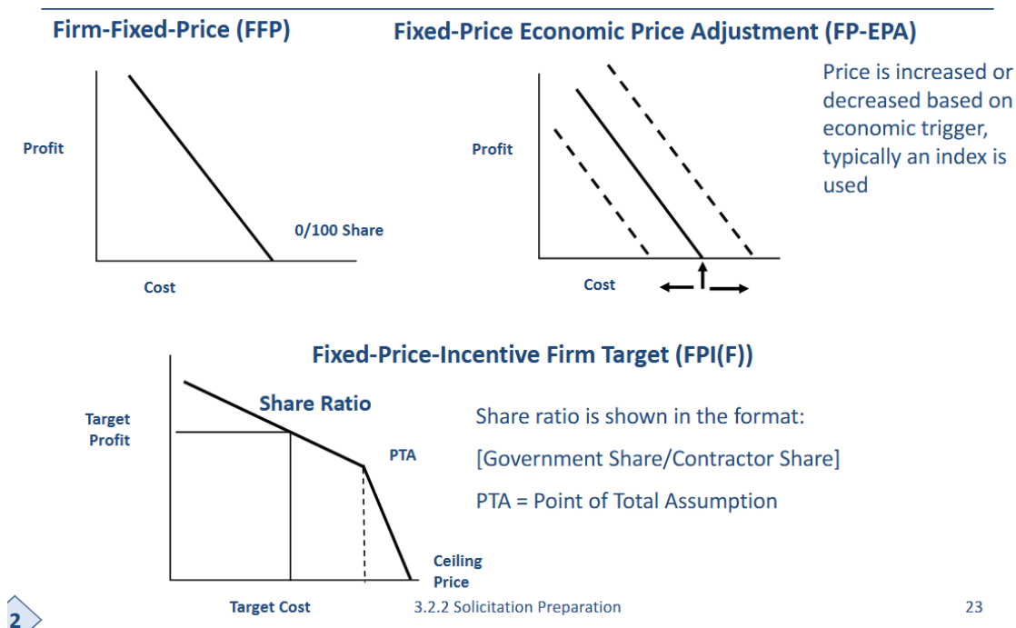
Figure 3.1. Fixed-price contract types and incentive geometry. Source: 3.2.2. Solicitation Preparation, 2026 [72].
