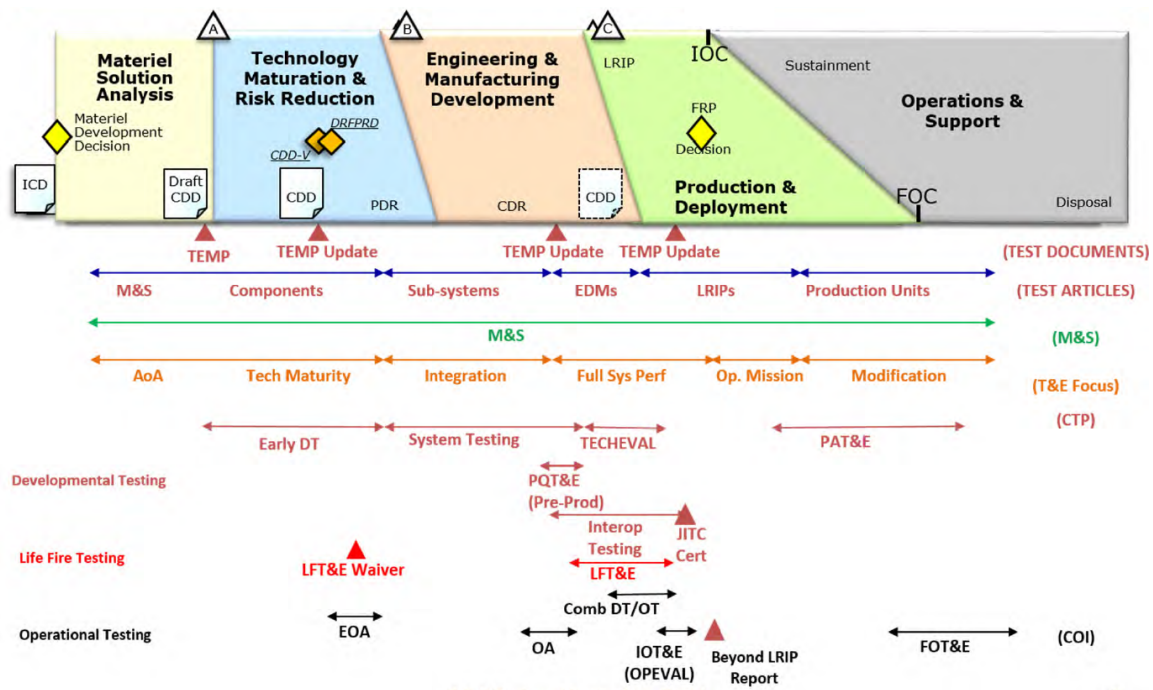
Figure 5.3. Key MCA test and evaluation touchpoints that frame DT, OT, and certification decisions. Source: 3.5.5. Test and Evaluation Part I, 2025 [170].
