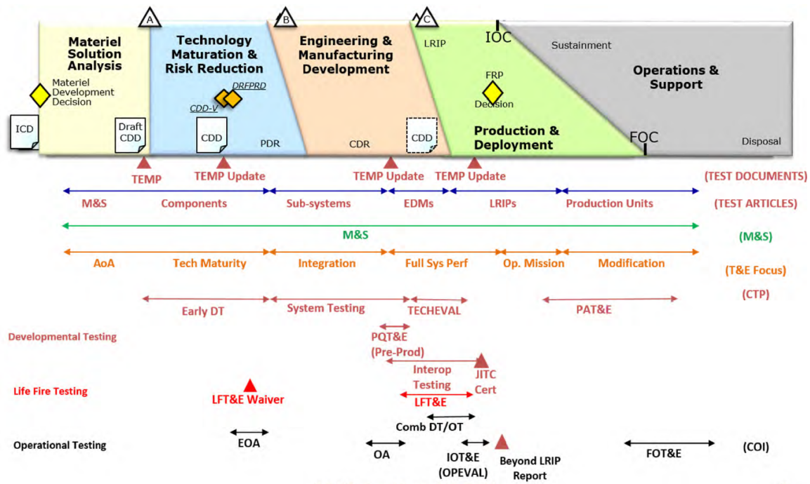
Figure 5.4. Key MCA test and evaluation touchpoints that frame DT, OT, and certification decisions. Source: 3.5.5. Test and Evaluation Part I, 2025 [74].
