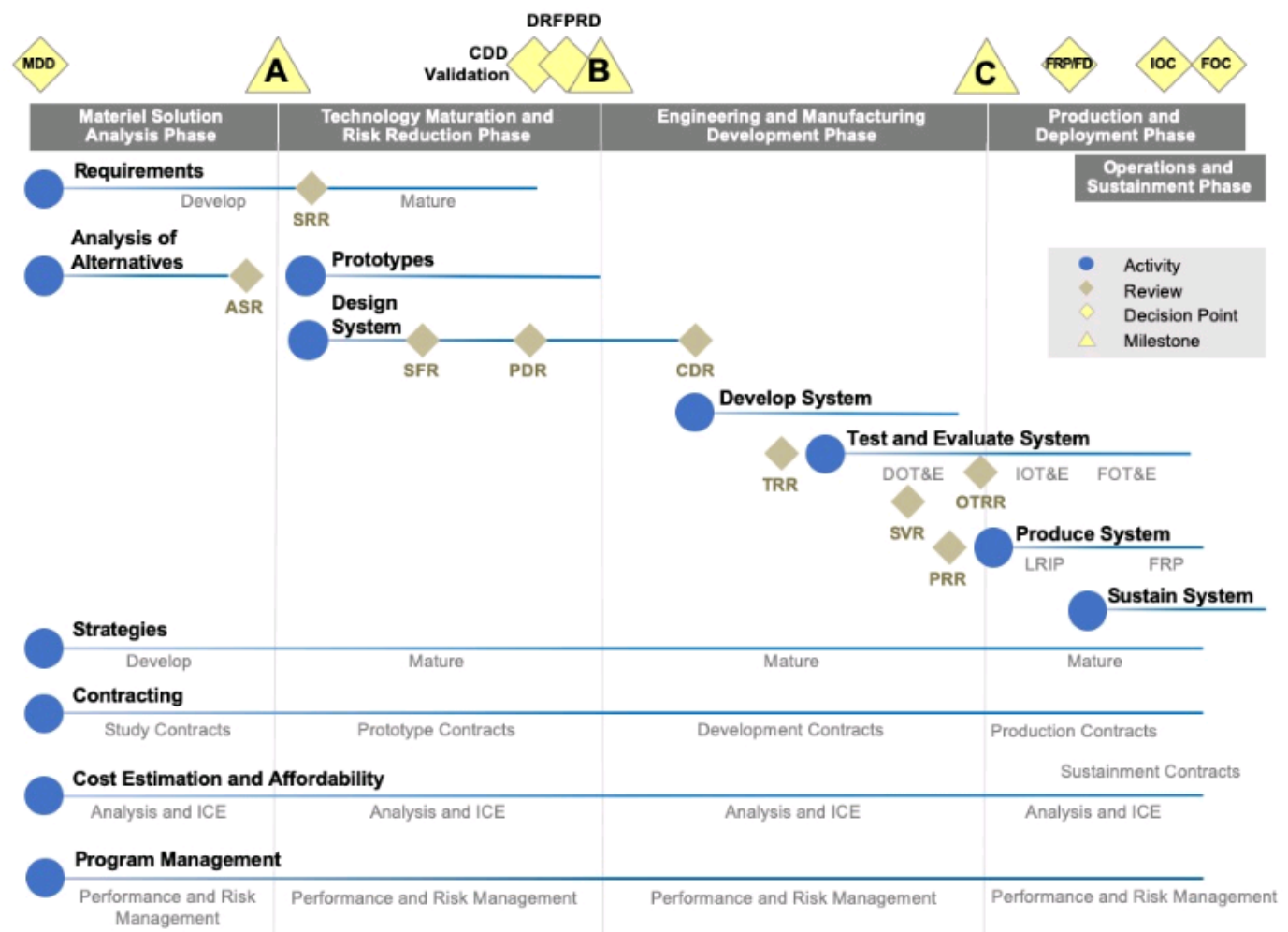
Figure 4.5. Lifecycle view for a MCA showing all functions and activities for each phase. Source: DoDI 5000.85, 2020 [33]
