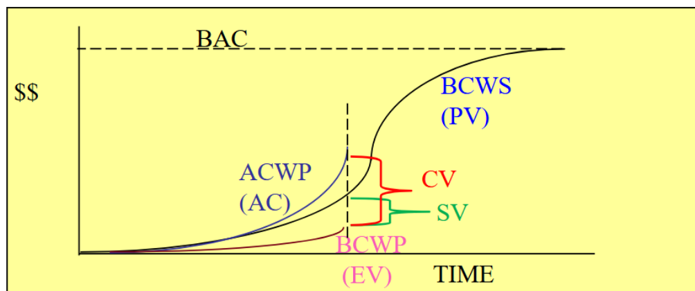
Figure 3.7. EVM chart showing the independent variables and variances. Source: edo-3-6-2-evm-analysis-2025, edo-3-6-2-evm-analysis-2025 [edo-3-6-2-
