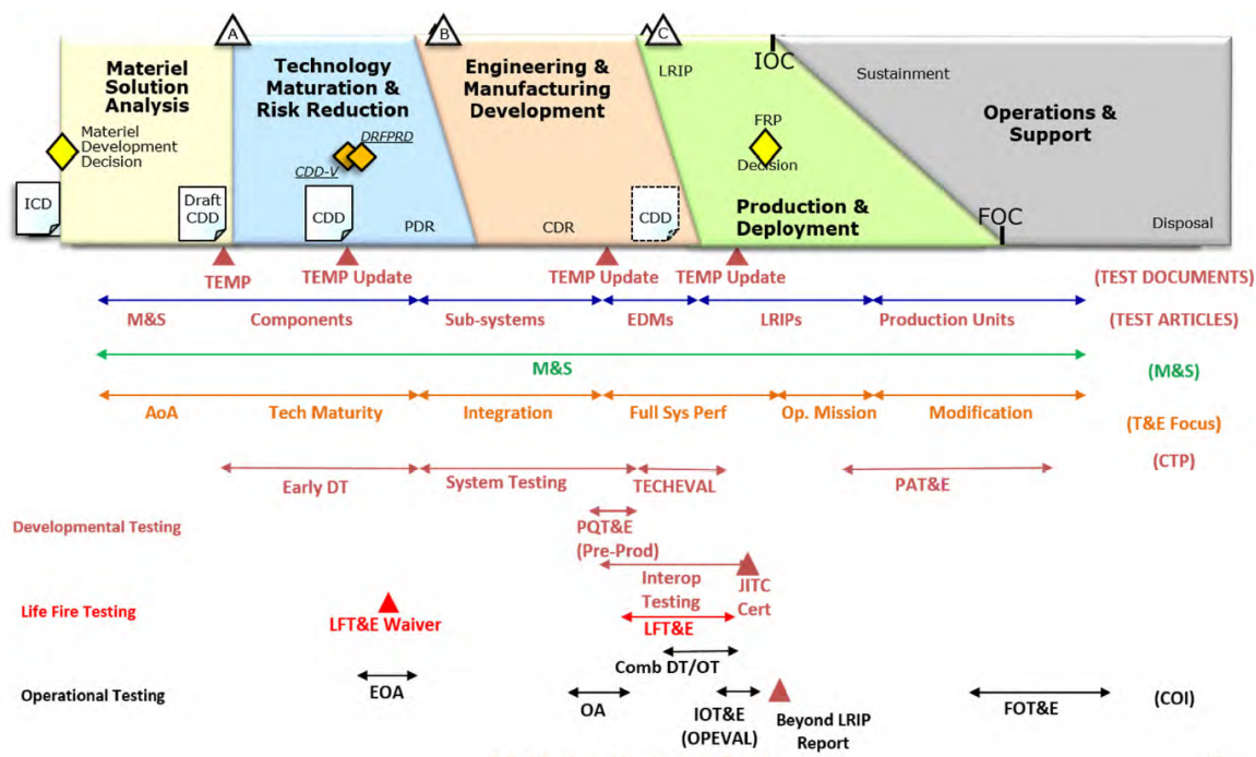
Figure 5.3. Key MCA test and evaluation touchpoints that frame DT, OT, and certification decisions. Source: 3.5.5. Test and Evaluation Part I, 2025 [204].
