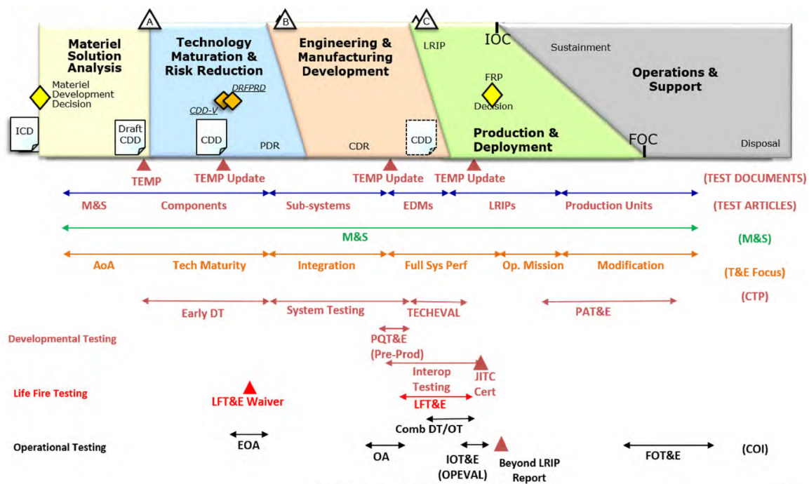
Figure 5.3. Key MCA test and evaluation touchpoints that frame DT, OT, and certification decisions. Source: 3.5.5. Test and Evaluation Part I, 2025 [279].
