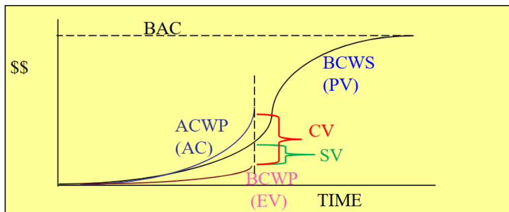
Figure 3.7. EVM chart showing the independent variables and variances. Source: 3.6.2. EVM Data Analysis, 2025 [50]
