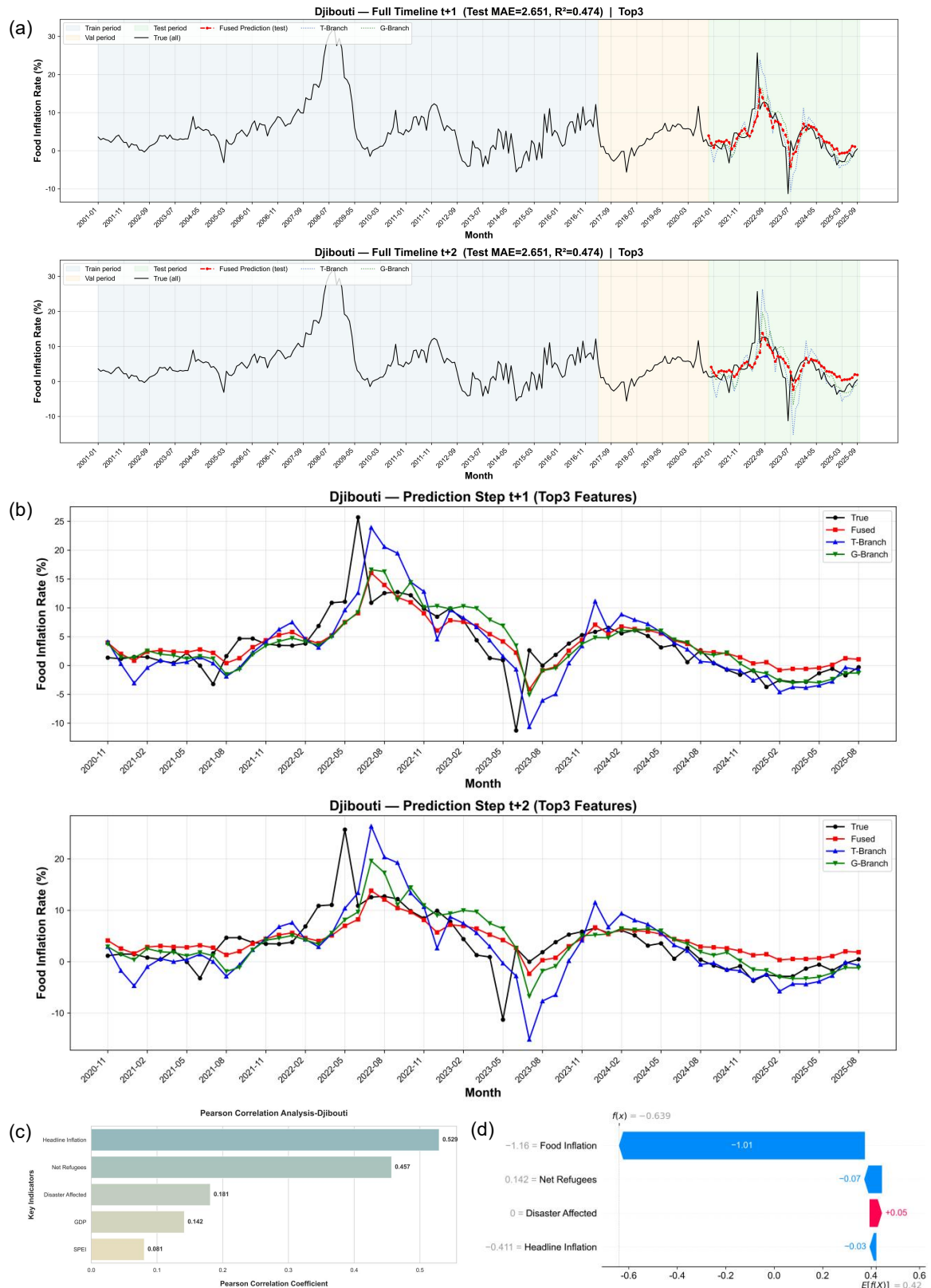
Multidimensional Evaluation and Attribution Analysis of Food Inflation Forecast in Djibouti. (a) Overview of the total cycle prediction and fitting. (b) Multi-step Short-Term Forecast Comparison Chart, (c) Pearson correlation analysis of macroeconomic drivers, (d) SHAP-based explanation of feature contributions for a specific prediction instance.
