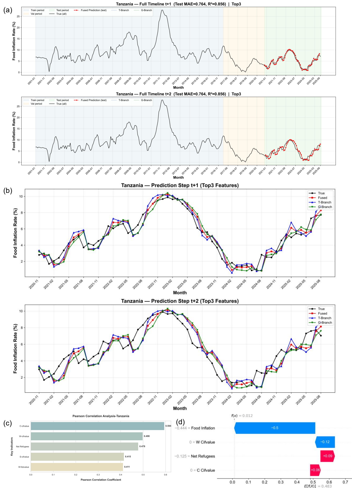
Multidimensional Evaluation and Attribution Analysis of Food Inflation Forecast in Tanzania. (a) Overview of the total cycle prediction and fitting, (b) Multi-step Short-Term Forecast Comparison Chart, (c) Pearson correlation analysis of macroeconomic drivers, (d) SHAP-based explanation of feature contributions for a specific prediction instance.
