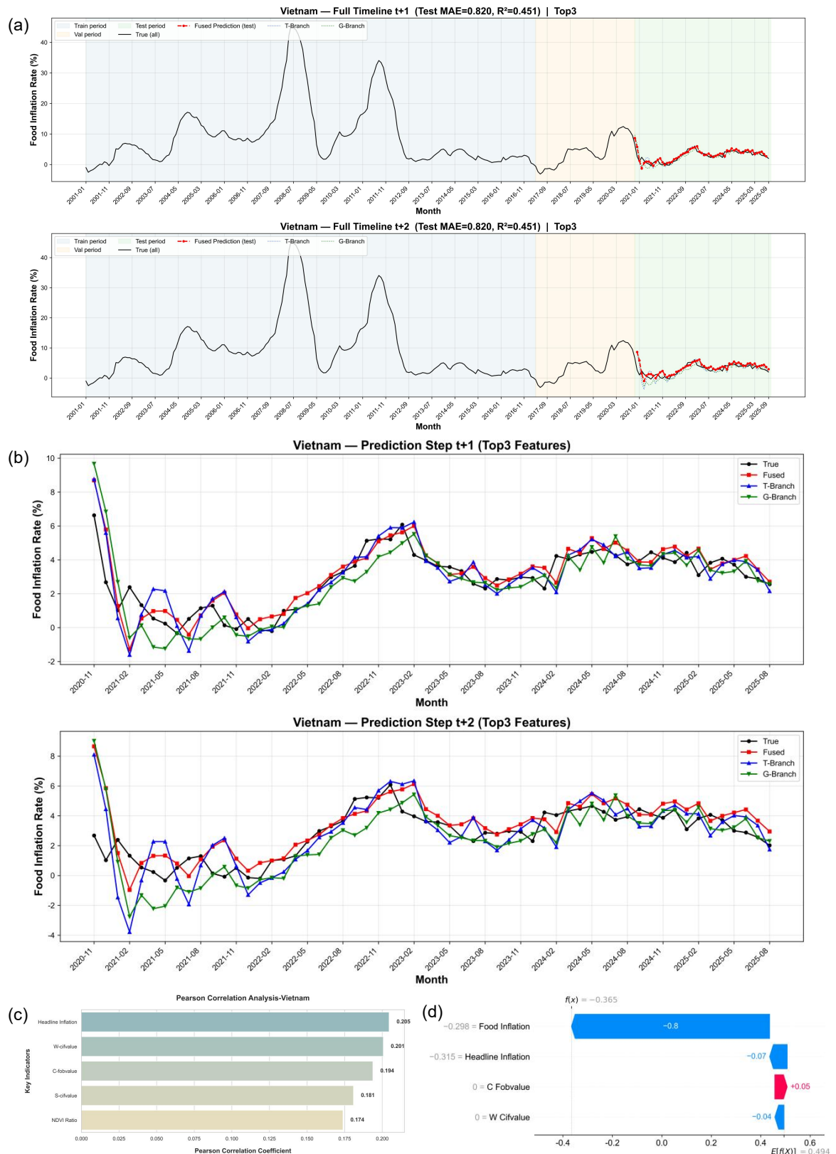
Multidimensional Evaluation and Attribution Analysis of Food Inflation Forecast in Vietnam. (a) Overview of the total cycle prediction and fitting, (b) Multi-step Short-Term Forecast Comparison Chart, (c) Pearson correlation analysis of macroeconomic drivers, (d) SHAP-based explanation of feature contributions for a specific prediction instance.
