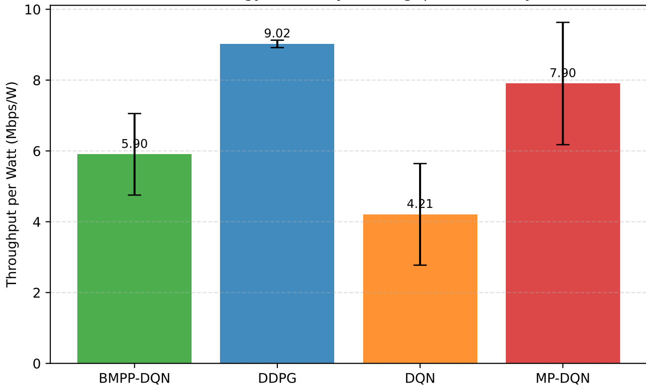
O-RAN Track: Energy Efficiency (Throughput/Power) by Method
