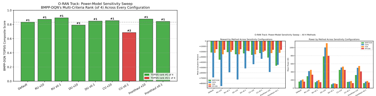
Figure 4.7: Pre-fix archive snapshot (not rerun against Section 4.2’s corrections). BMPP-DQN’s TOPSIS score/rank (left) and reward/power for all 4 methods (right), across the default configuration and all 8 perturbed power-model configurations, under the environment as it existed before the fixes.
