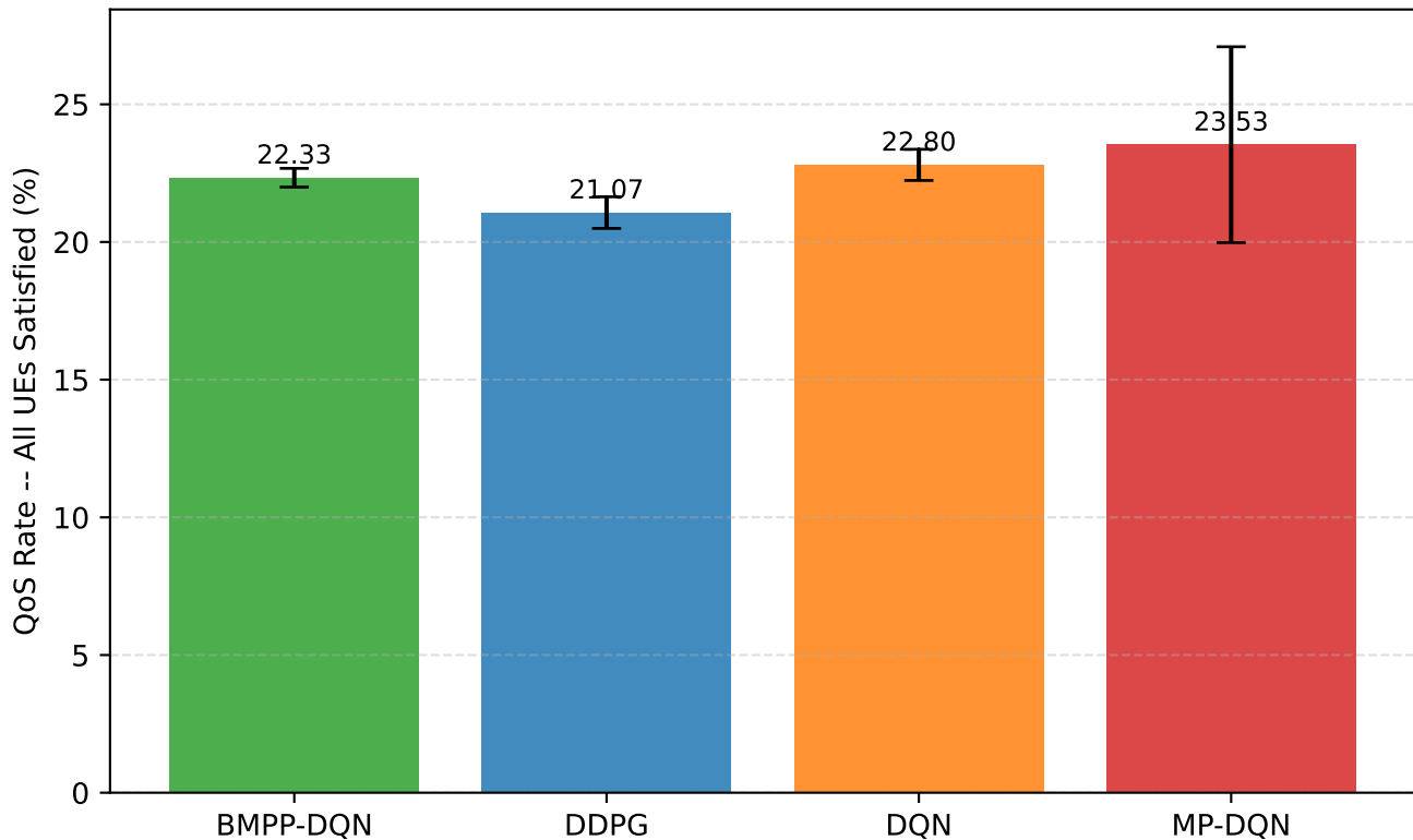
O-RAN Track: QoS Rate -- All UEs Satisfied (%) by Method
