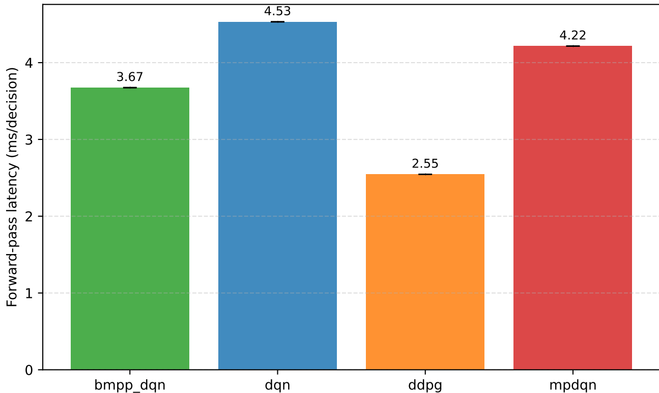
O-RAN Track: Inference-Time Latency Comparison
