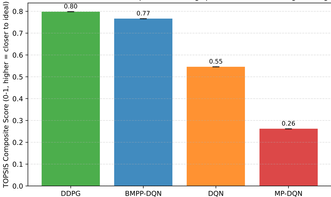
O-RAN Track: Multi-Criteria Composite Ranking (power, QoS, switching, throughput)
