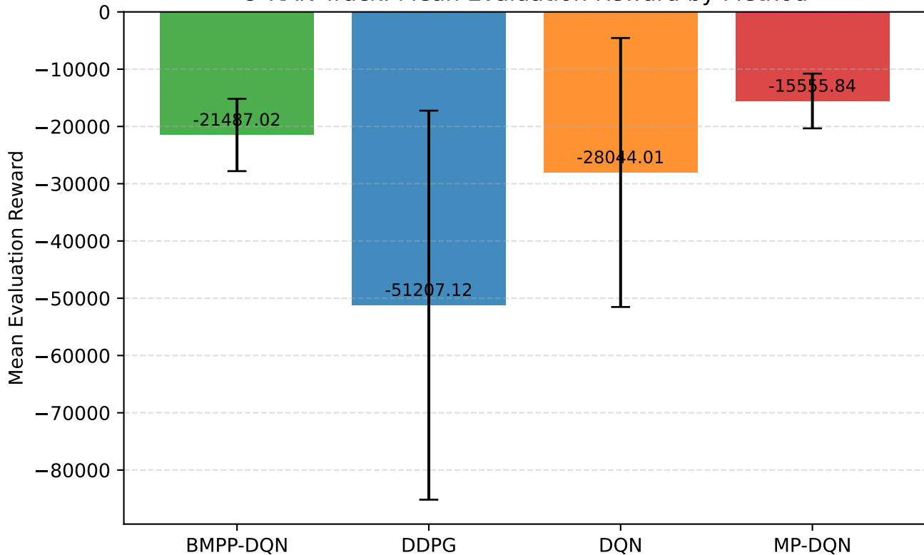
O-RAN Track: Mean Evaluation Reward by Method
