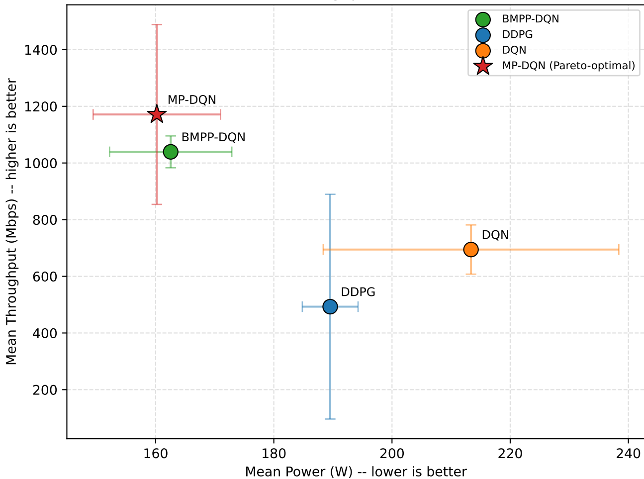
O-RAN Track: Power-Throughput Trade-off (Pareto Frontier)
