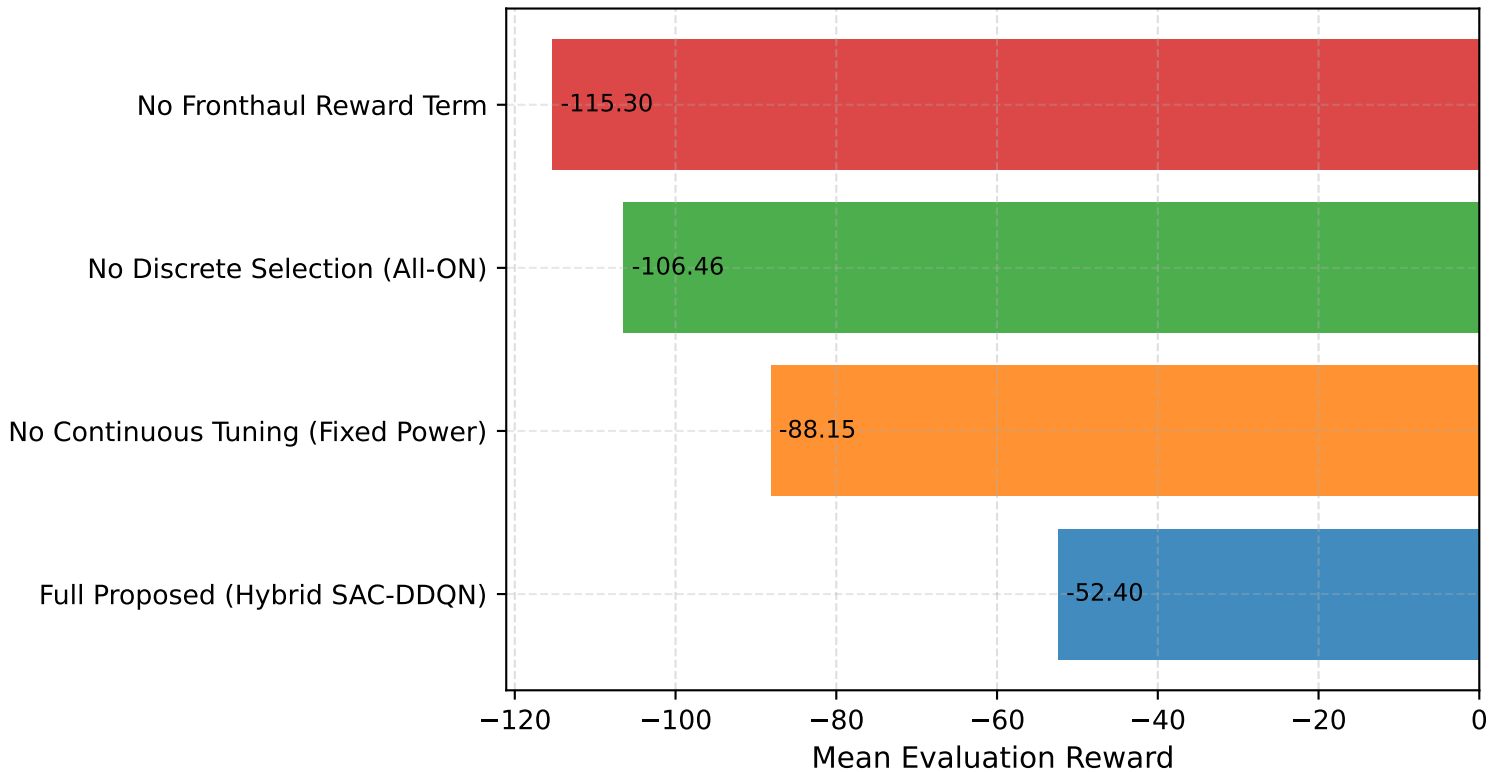
Ablation Study: Architecture Component Contributions
