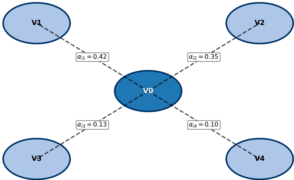
Figure 3: Multi-Head GAT Graph Attention Mechanism (Attention Weights \alpha )
