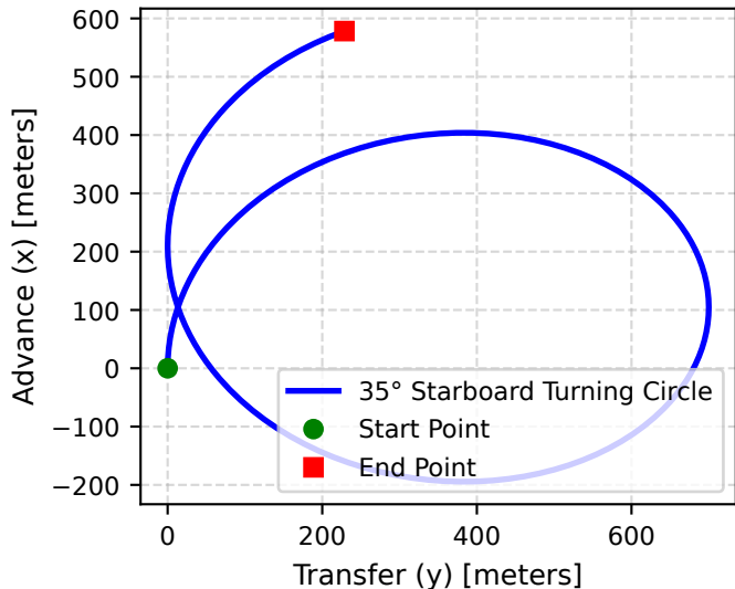
3-DOF MMG Turning Circle (IMO Standard)
