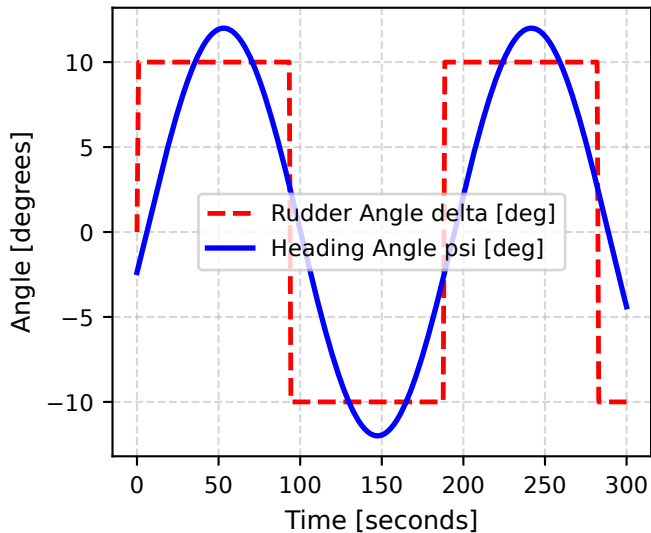
10°/10° Zig-Zag Maneuver Response
