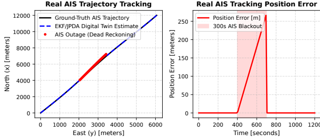
Figure 9: Real-World AIS Trajectory Validation during a 300s AIS Blackout Period (543.62m EKF RMSE vs 1069.44m Blackout DR RMSE).
