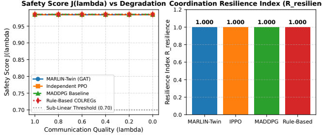
Figure 8: Baseline Algorithm Coordination Resilience Comparison. MARLIN-Twin maintains R_{\text{resilience}} = 1.0000 across all bandwidth degradation levels ( \lambda ).
