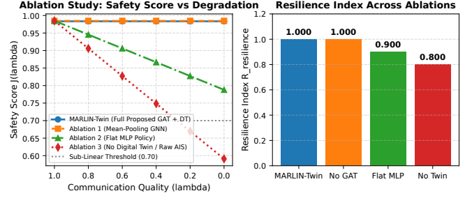
Figure 10: 4-Variant Model Ablation Study comparing MARLIN-Twin against Mean-Pooling GNN, Flat MLP, and No Digital Twin variants.
