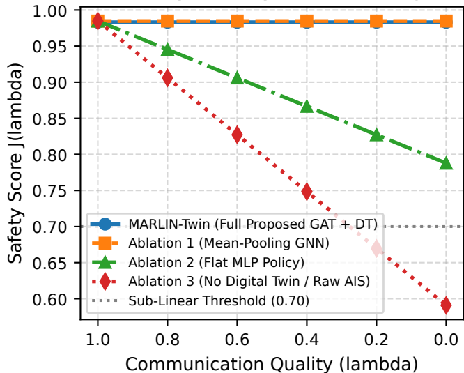
Ablation Study: Safety Score vs Degradation
