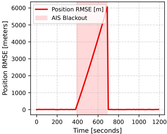
Position Tracking Error Over Time
