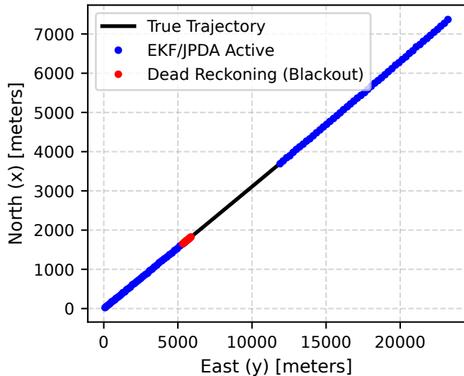
Digital Twin EKF/JPDA Trajectory Estimate
