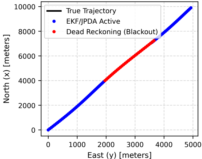
Digital Twin EKF/JPDA Trajectory Estimate
