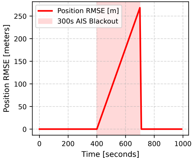
Position Tracking Error Over Time
