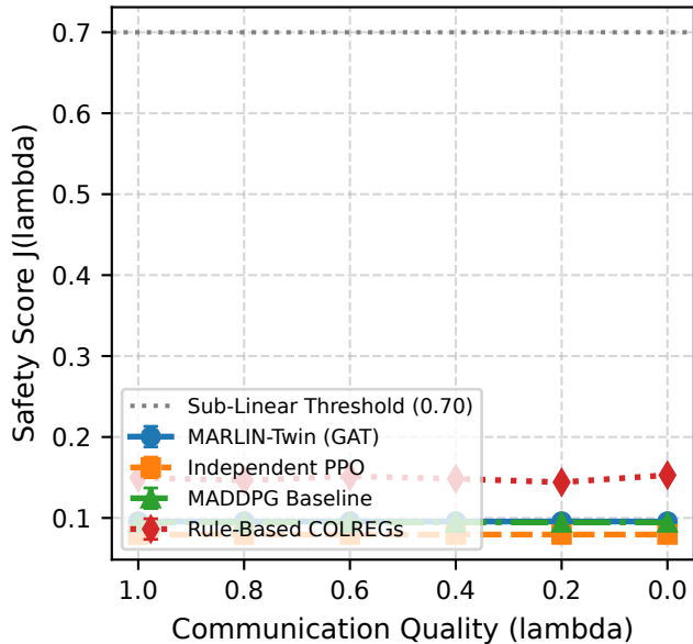
Safety Score J(\lambda) vs Degradation
