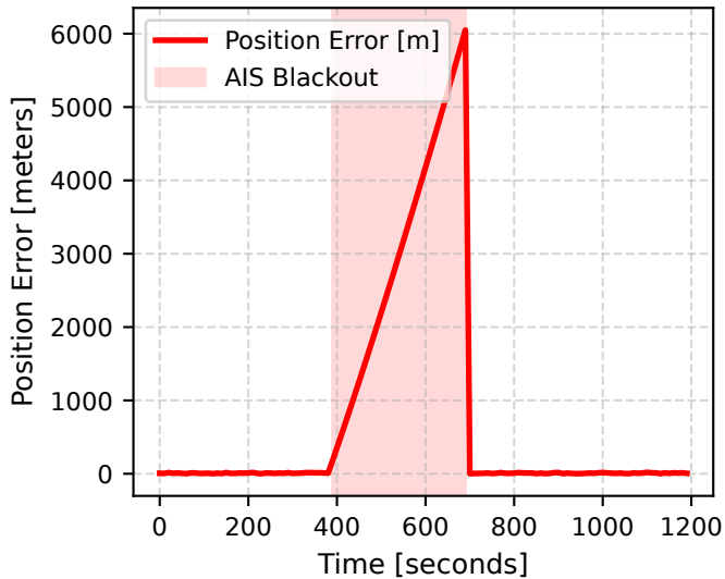
Simulated AIS Tracking Position Error
