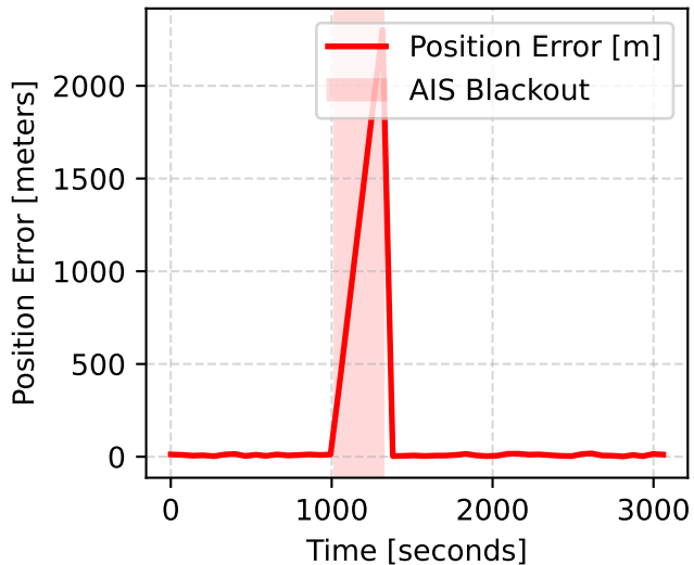
Real AIS Tracking Position Error
