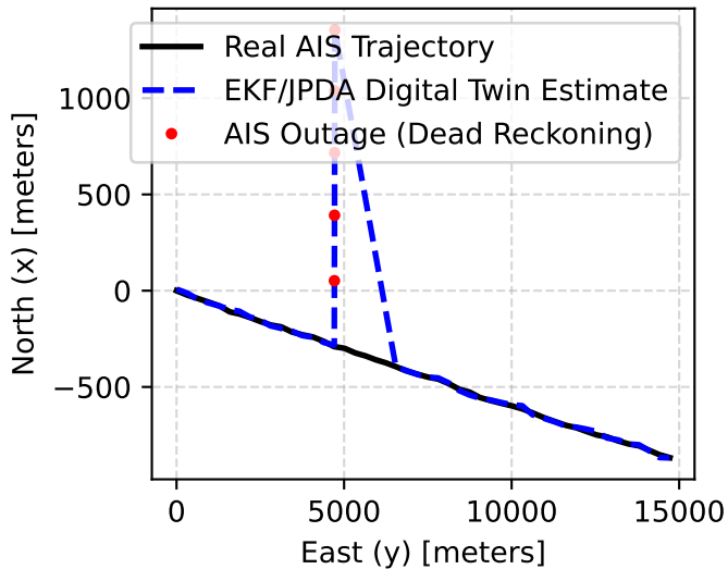
Real AIS Trajectory Tracking
