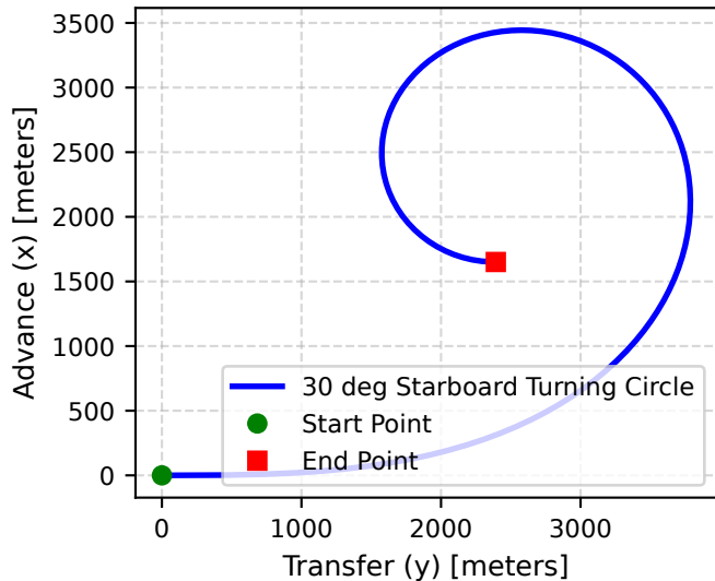
3-DOF MMG Turning Circle (IMO Standard)
