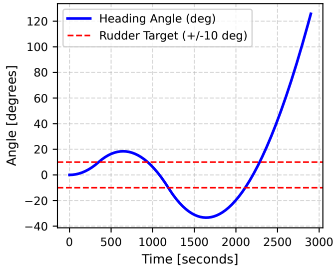
10/10 Zig-Zag Maneuver Response
