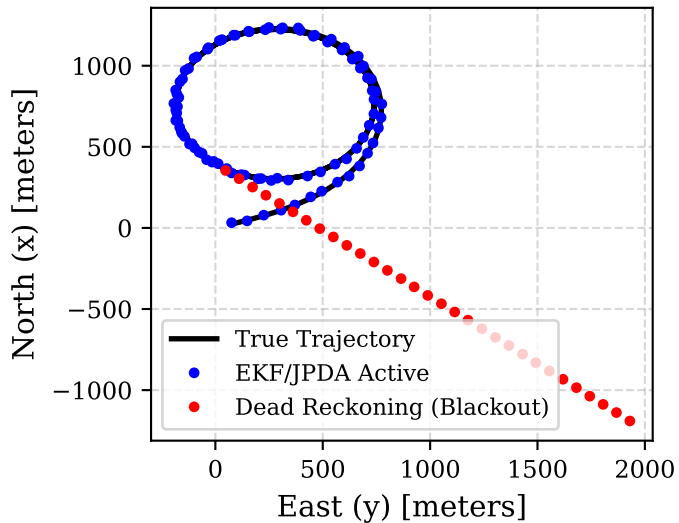
Digital Twin EKF/JPDA Trajectory Estimation
