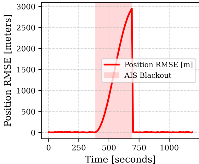
Digital Twin EKF/JPDA Trajectory Estimation
