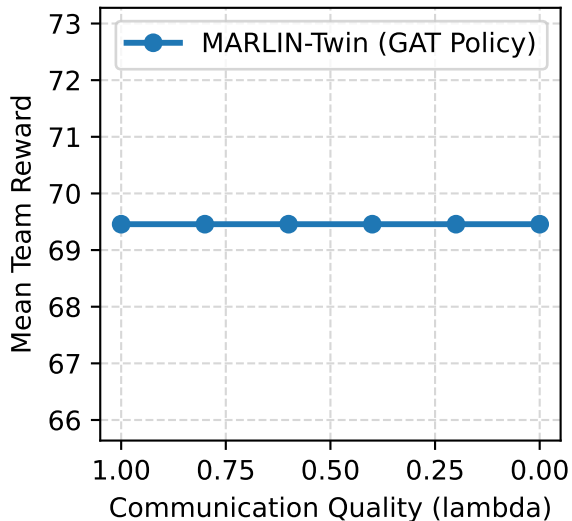
Reward vs. Bandwidth Quality \lambda
