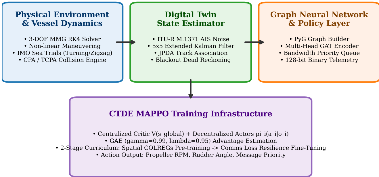
Figure 1: MARLIN-Twin Overall System Architecture Block Diagram
