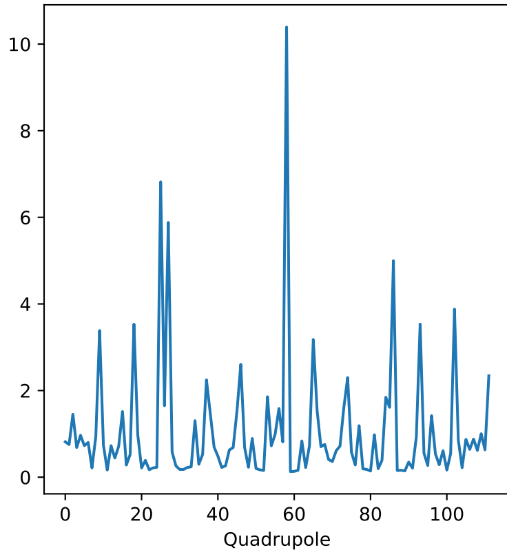
Vertical direction, Total = 0.3840\%
