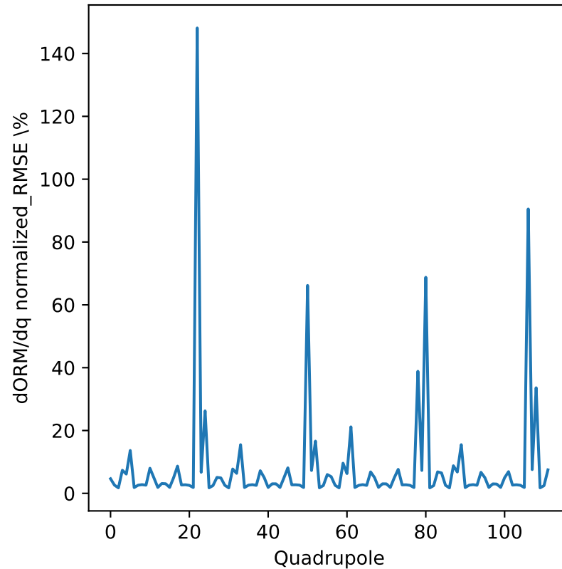
Horizontal direction, Total = 1.8183\%
