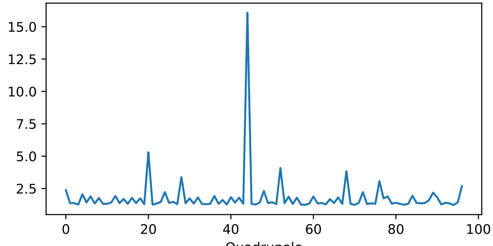
Vertical direction, Total RMSD = 1.5795\%
