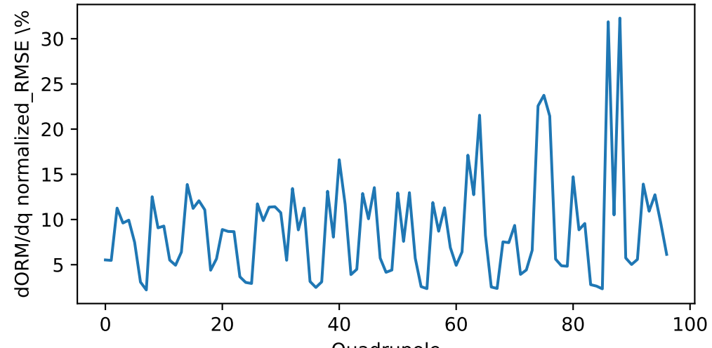
Horizontal direction, Total RMSD = 4.9290\%
