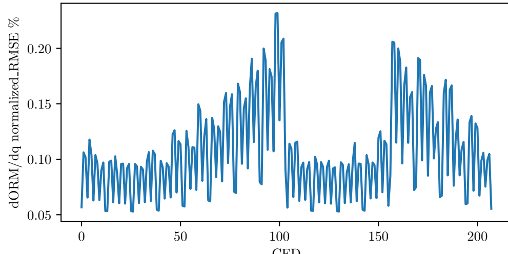
Horizontal direction, Total RMSD = 0.0731%
