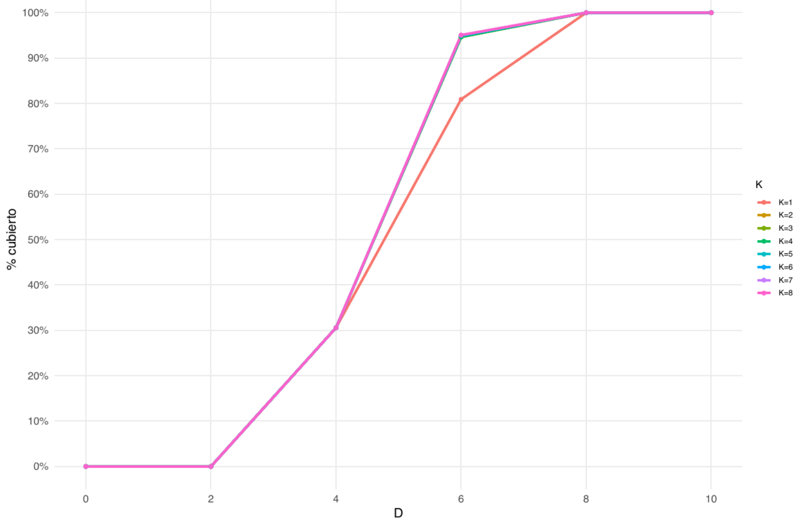
greedy – ext – 100–9
