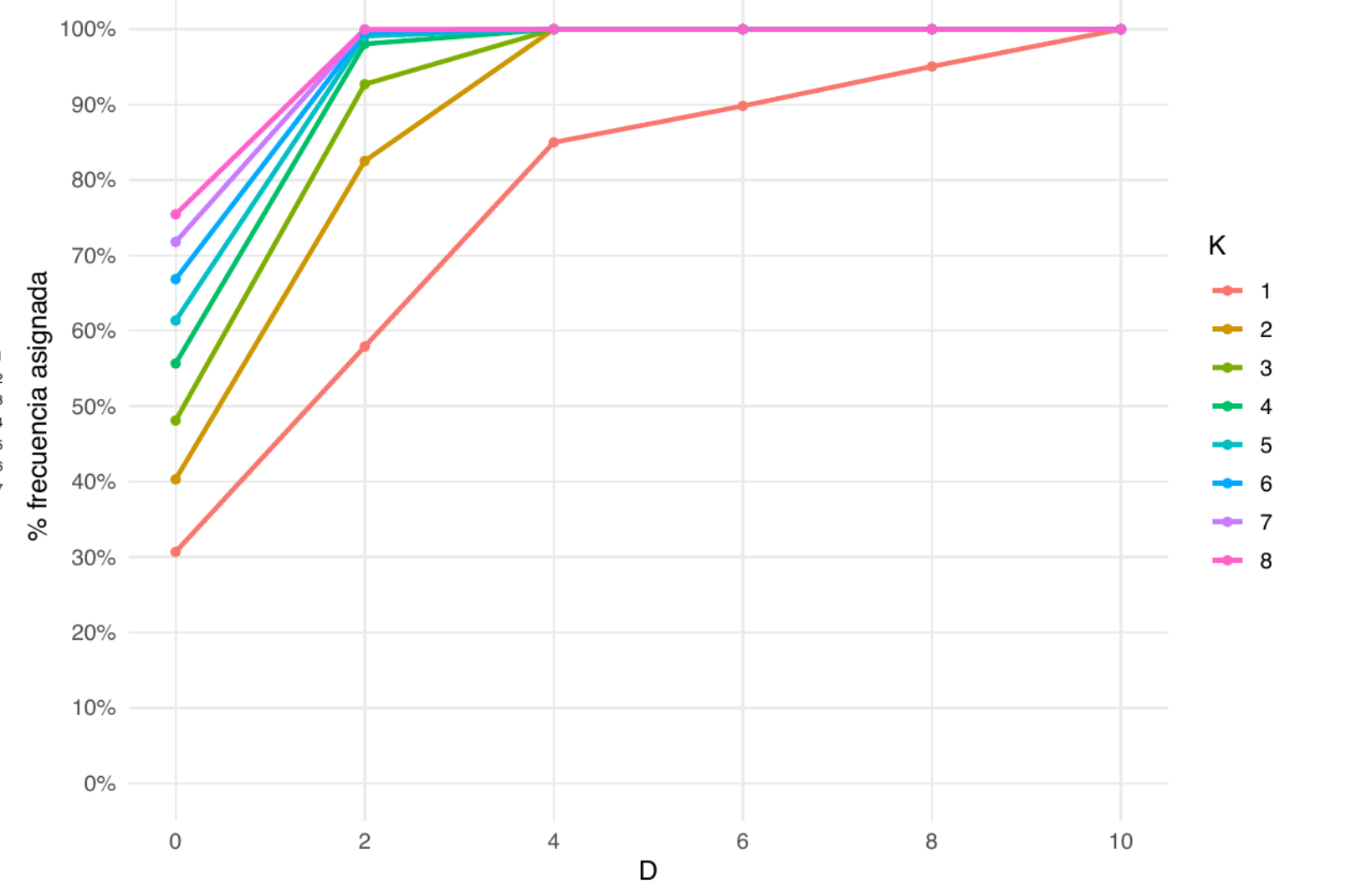
greedy – ext – 100–9
