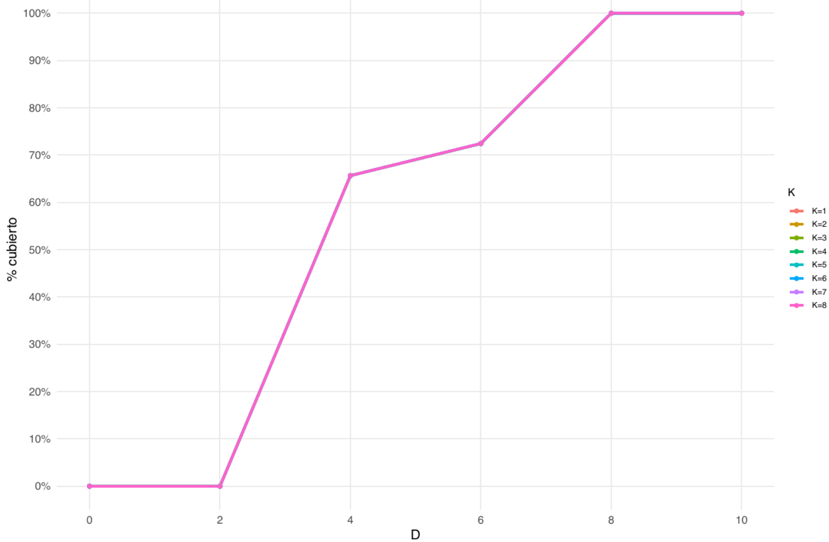
greedy – pos – 10–9
