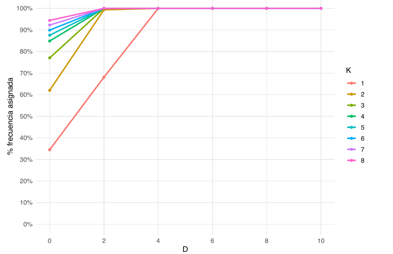
greedy – pos – 10–9
