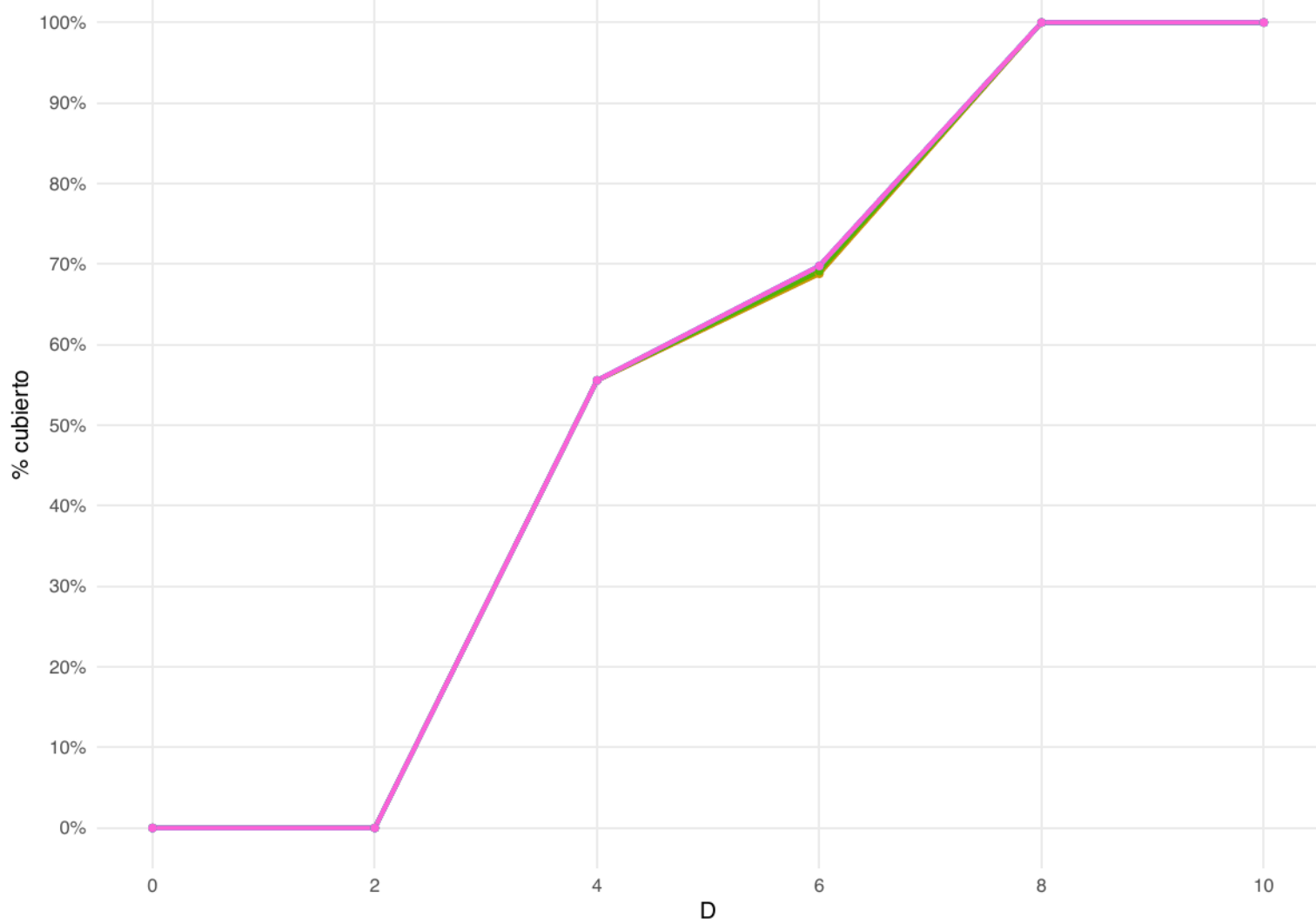
sins – pos – 10–9 (orden D=4)
