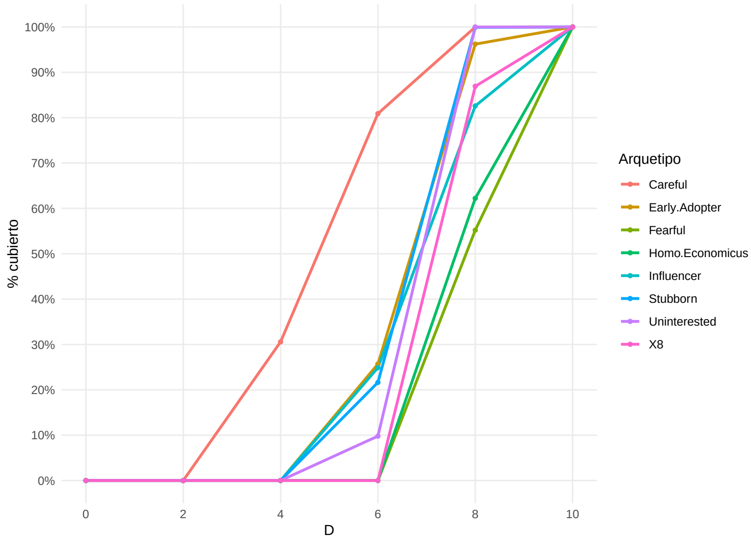
kmeans - ext - 100-9
