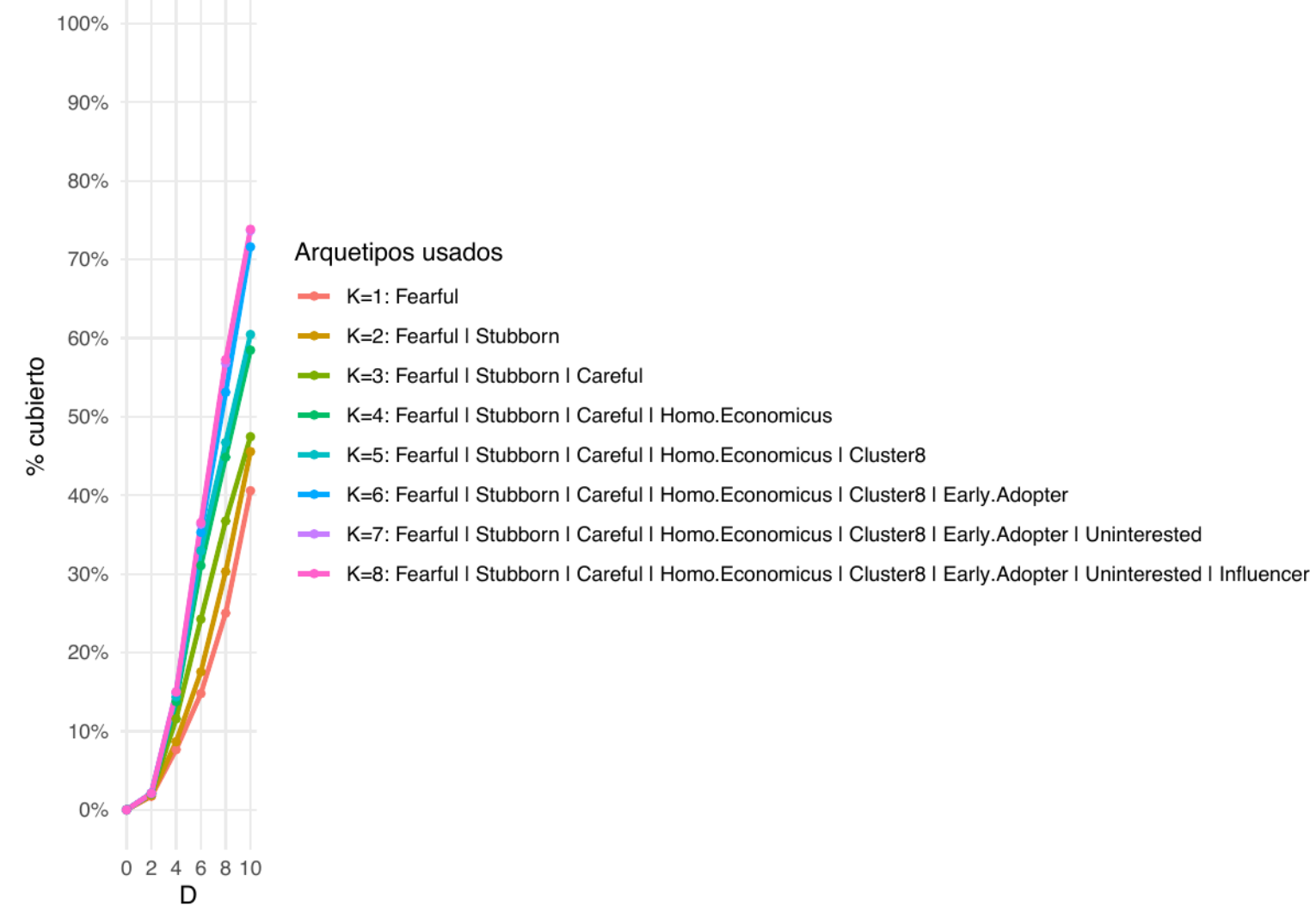
greedy – ext – 10–32
