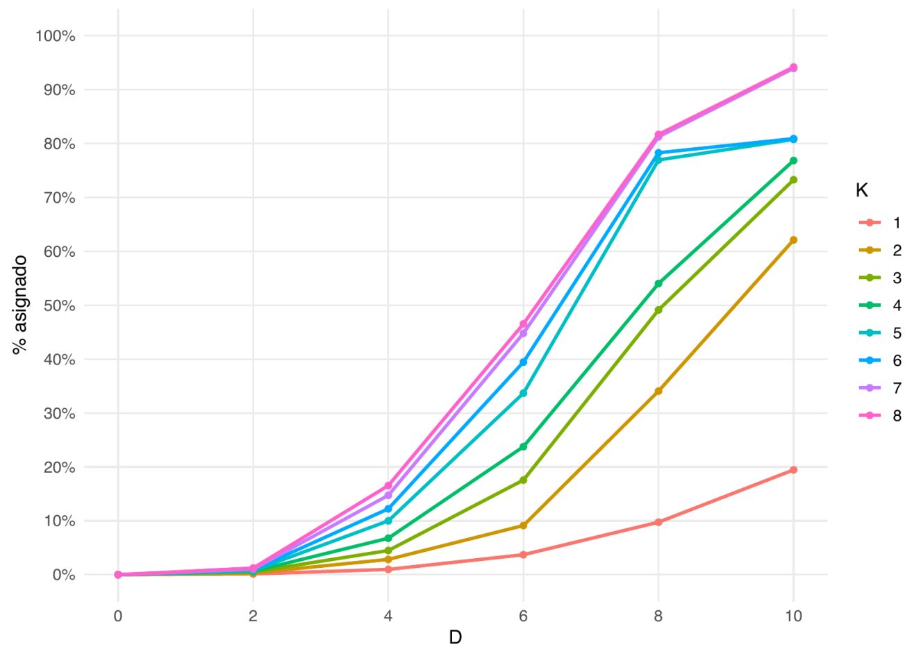
greedy – ext – 10–32
