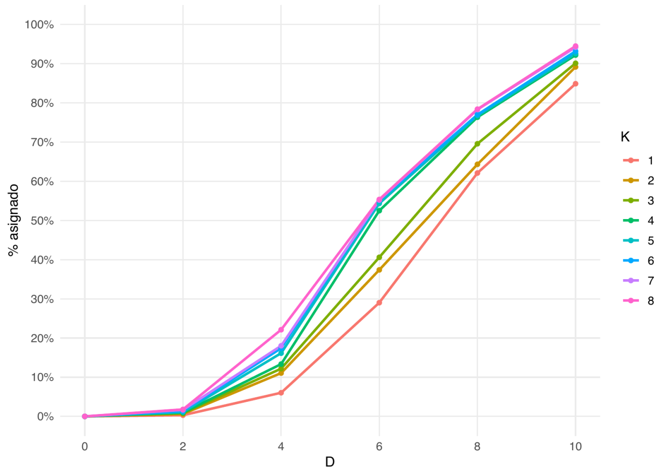
greedy – pos – 10–32
