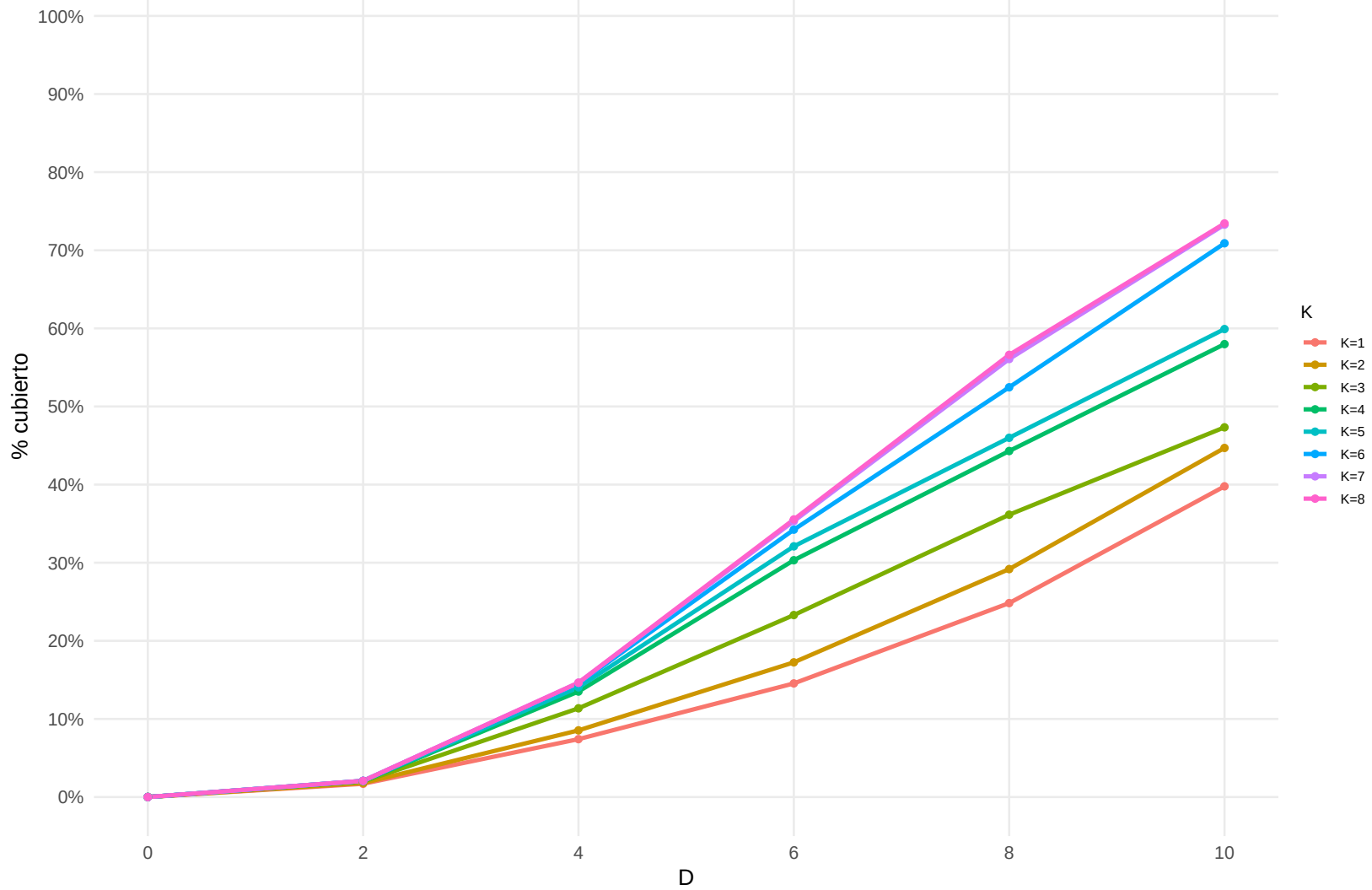
kmeans - ext - 100-32 (orden D=4)
