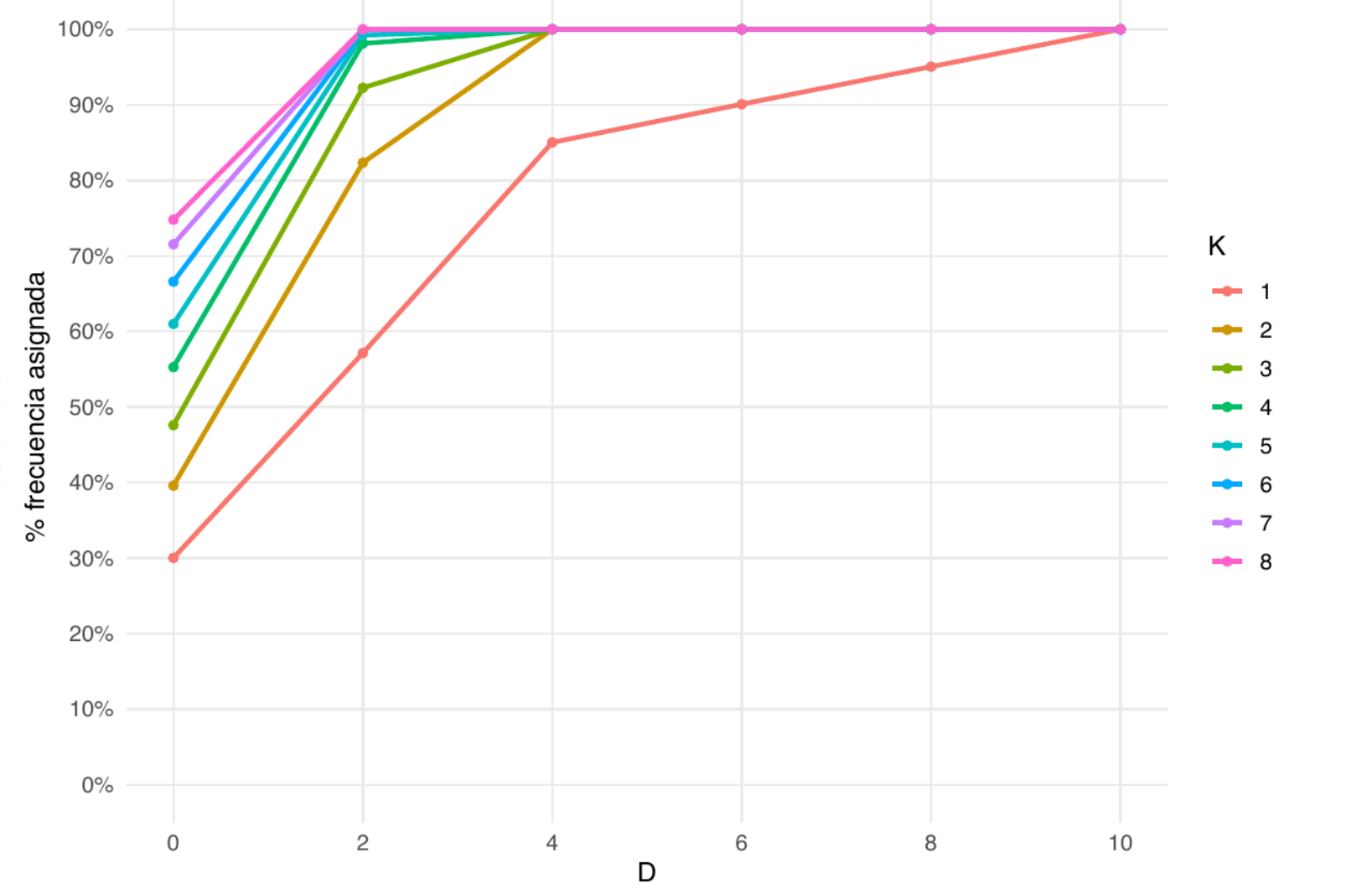
greedy – ext – 10–9
