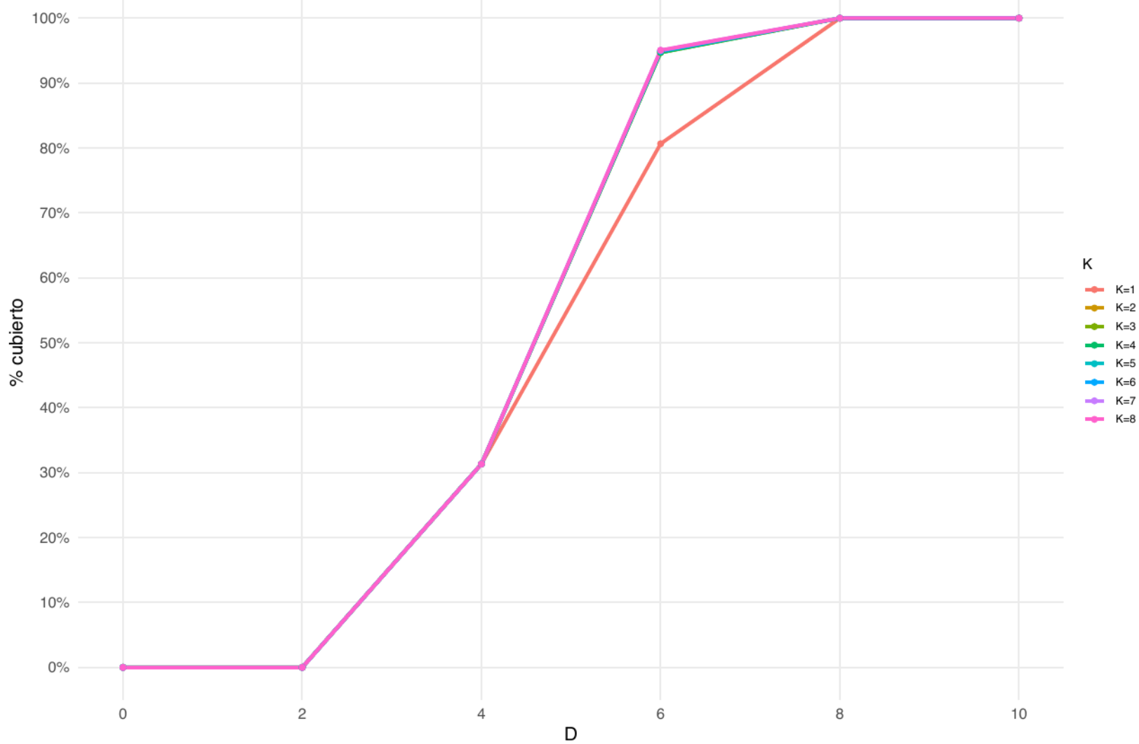
greedy – ext – 10–9
