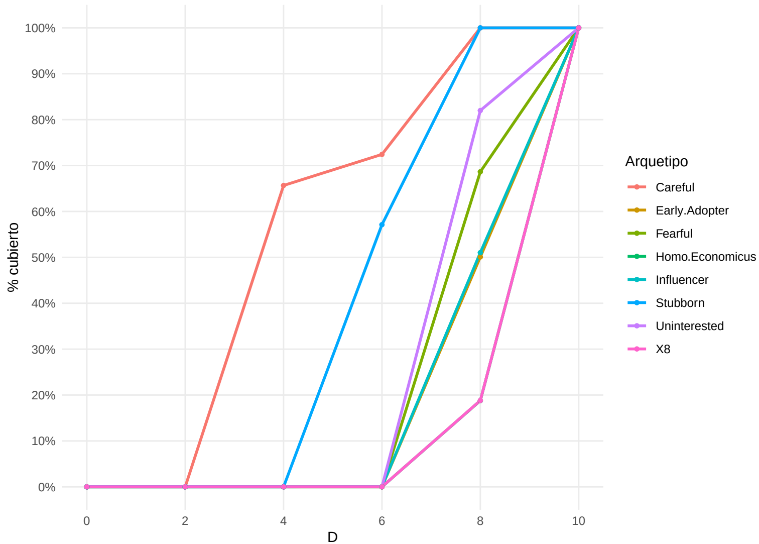
kmeans - pos - 10-9
