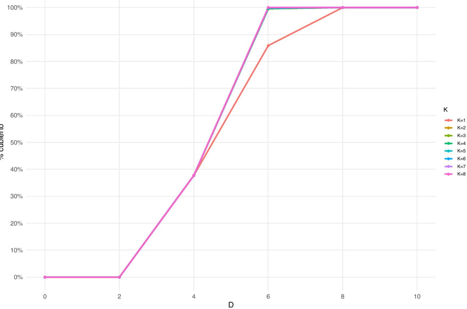
greedy – ext – 100–9–top3
