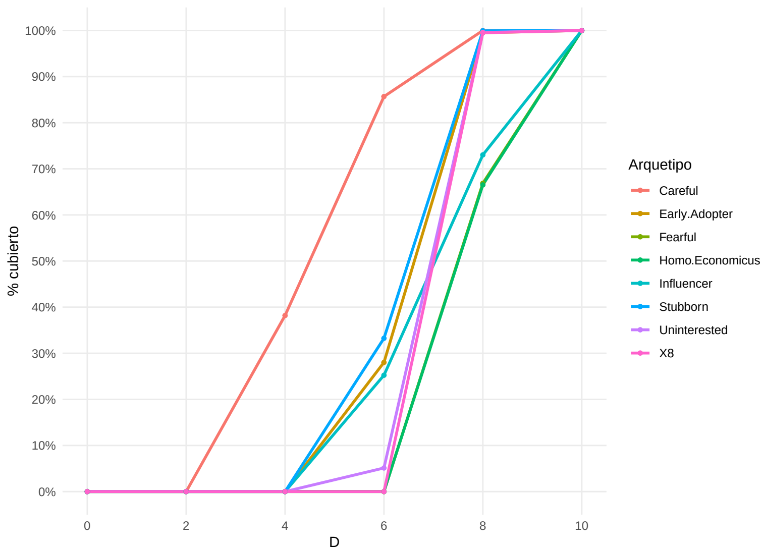
kmeans - ext - 10-9-top3
