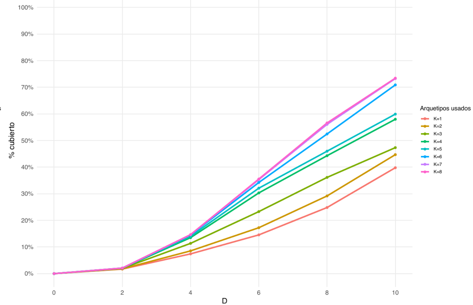
greedy – ext – 100–32
