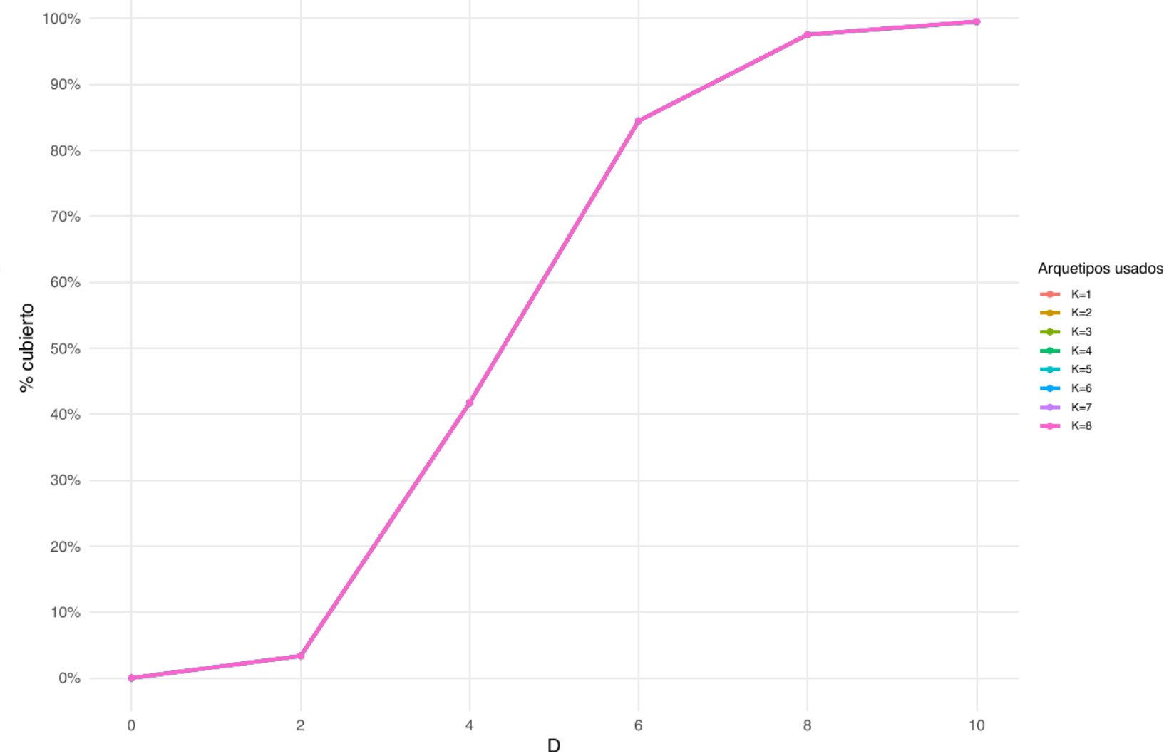
greedy – pos – 10–32
